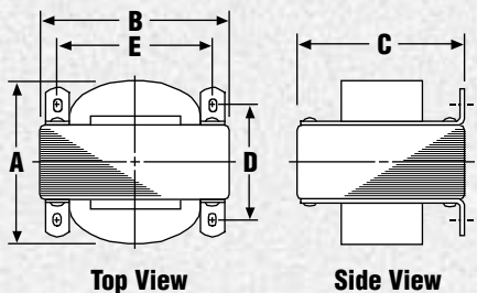
Figure C Class 105° C Insulation System 55° C Temperature Rise Epoxy Encapsulated Coils
