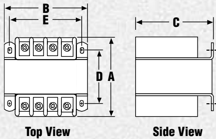
Figure A Class 105° C Insulation System 55° C Temperature Rise Epoxy Encapsulated Coils
